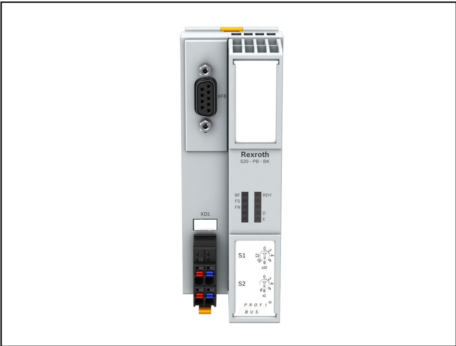
Fig. 5-7: Rexroth Profibus bus coupler S20-PB-BK The bus coupler is intended for use within a Profibus network and is the link to the IndraControl S20 system. It is modular extendable with S20 modules. Using the bus coupler, up to 63 S20 devices can be connected to an existing Profibus network.
