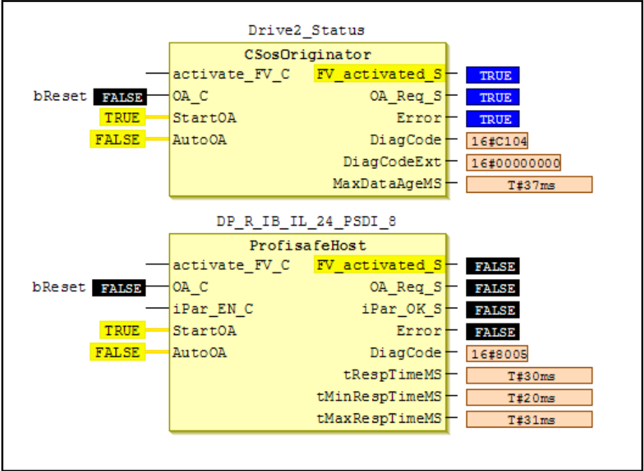
Fig. 8-12: Example call of the CsosOriginator and of the ProfisafeHost function block
