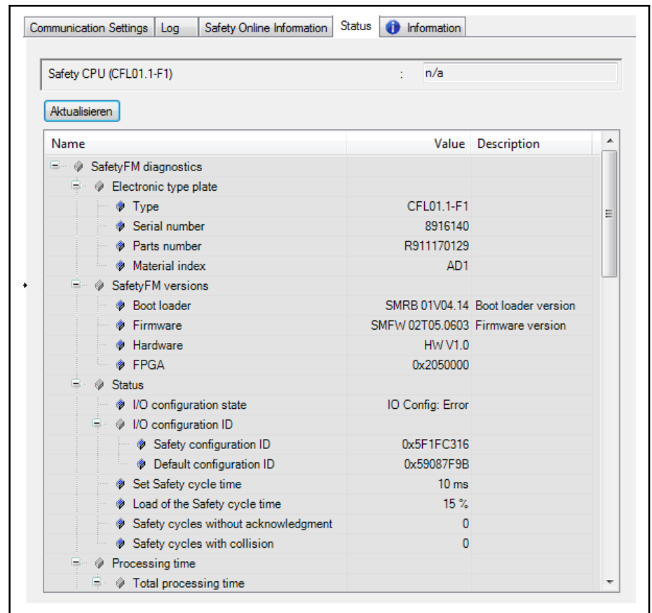
Fig. 8-1: Device status display (example: Safety function module)
