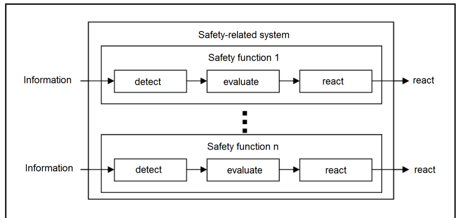
Fig. 3-2: Safety functions in the safety-related control system
