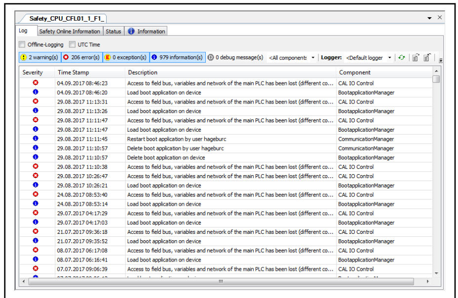
Fig. 8-3: Safety control logbook
