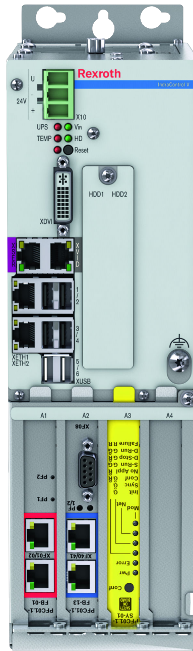
Fig. 4-5: Extension card PFC01.1-SY-01 in an IndraControl V
