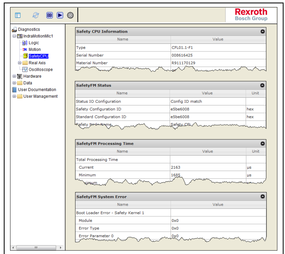
Fig. 8-11: Diagnostic display of the Safety function module
