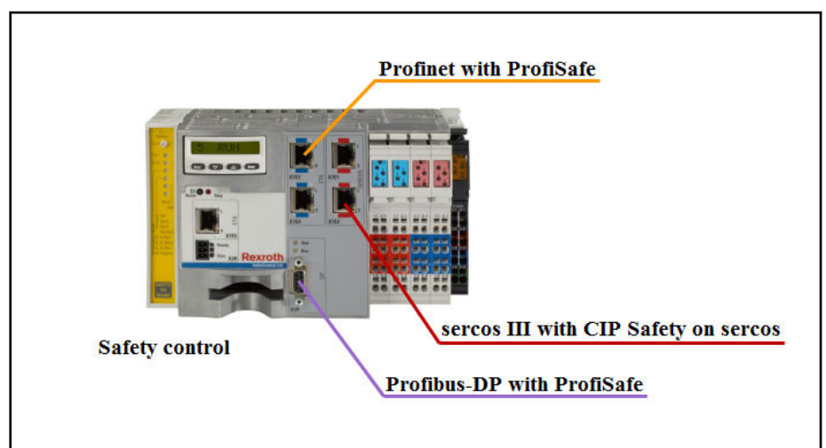
Fig. 4-7: Safe communication interface
