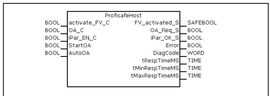
Fig. 5-13: Interface ProfisafeHost function block
