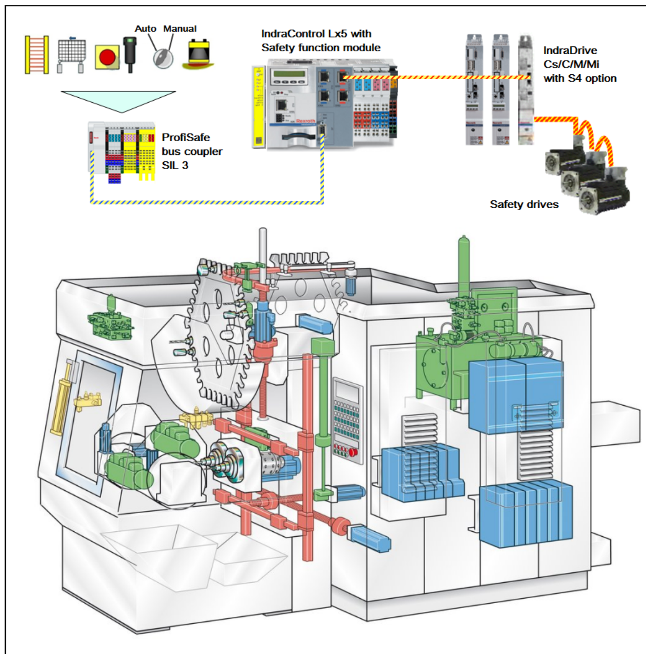
Fig. 4-8: Example IndraMotion MTX machining center
