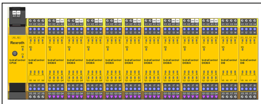
Fig. 4-6: Maximum setup of a SafeLogic compact system (without relay output extensions and gateways)
