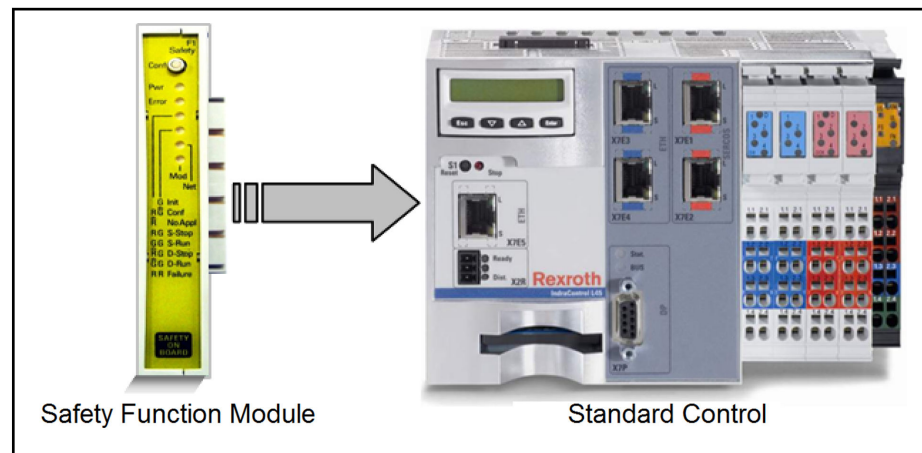
Fig. 4-4: Function module "Safety CPU (CFL01.1-F1)" for IndraControl Lxx controls
