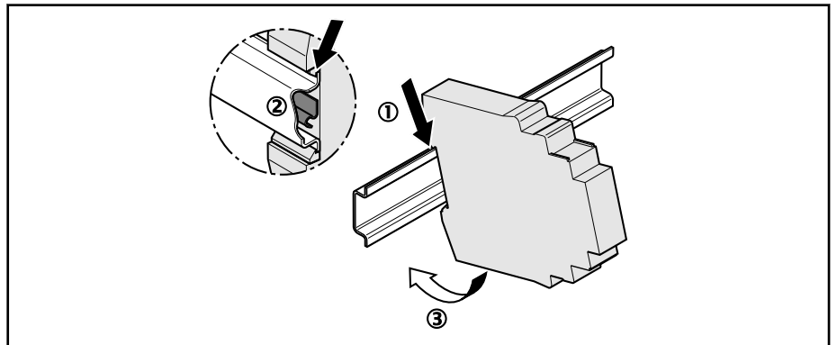
Fig. 7-3: Placing the module on the rail
