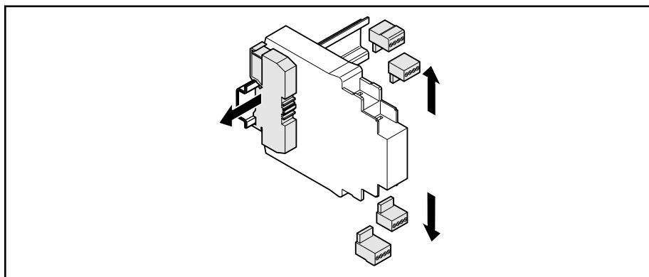
Fig. 7-5: Removing plug-in terminal blocks
