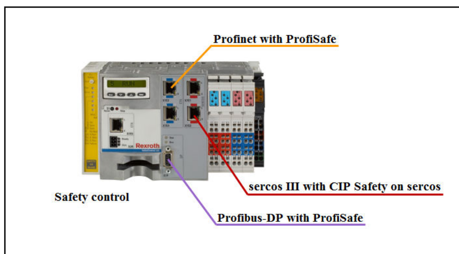
Fig. 4-5: Safe communication interface
