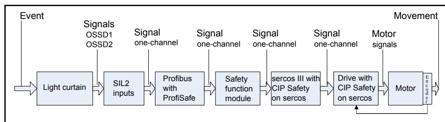
Fig. 3-17: Considered safety chain
