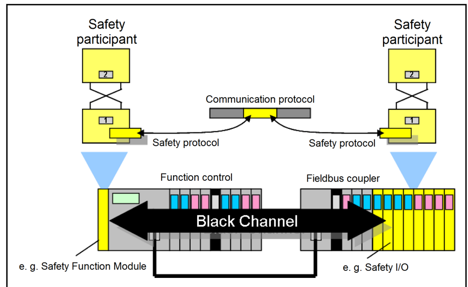
Fig. 4-7: Functional principle
