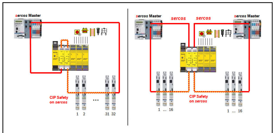
Fig. 4-1: Example topologies of SafeLogic compact with Sercos
