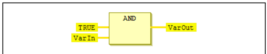
Fig. 6-11: Example of safe data flow: Operator AND with constant: TRUE, SAFE variables: VarIn and VarOut
