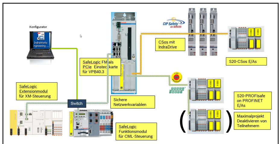
Fig. 4-2: System overview SafeLogic
