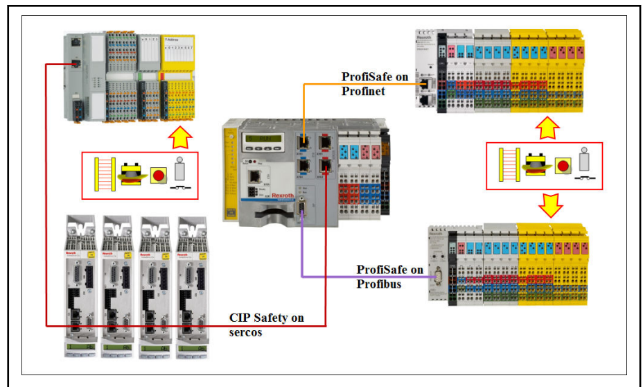
Fig. 3-8: Topology of a safety-related control system
