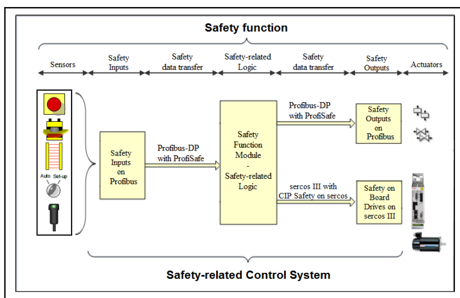
Fig. 3-9: Safety-related control system
