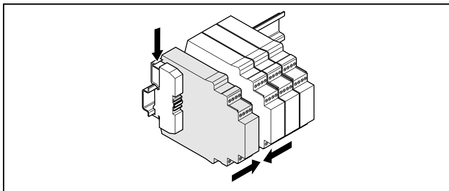
Fig. 7-4: Installing end brackets
