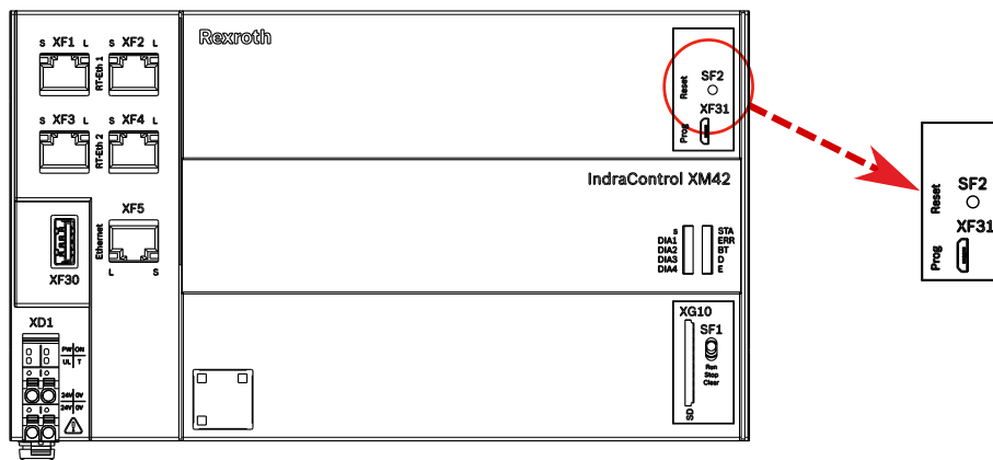
Abb. 12-5: Reset-Taster
