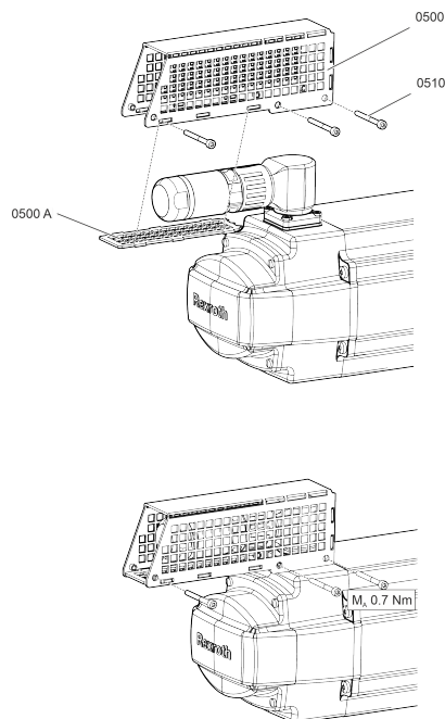
Fig. 17: Assemble plug connector protective cover M23
