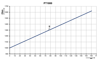
Fig. 3: Characteristic curve PT1000
