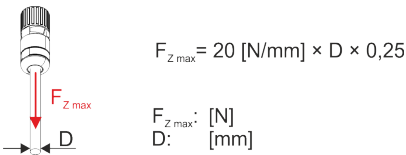
Fig. 1: Determination of maximum tensile load of connection cables
