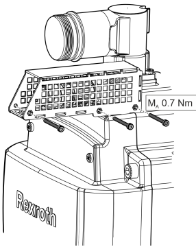
Fig. 16: Assemble plug connector protective cover M17
