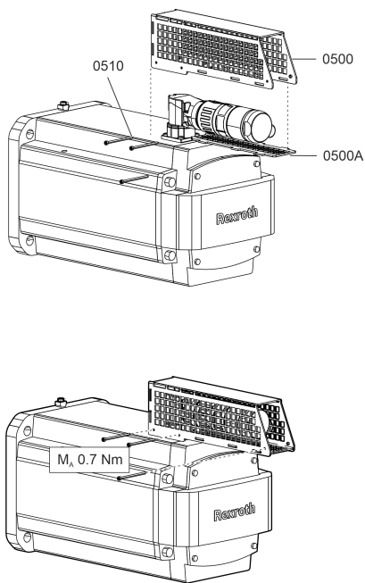
Fig. 18: Plug connector protective cover M40 assembly
