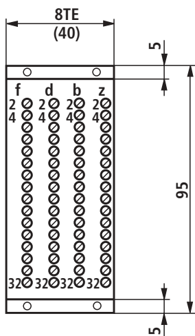
Adapter, 64-polig, Bauform G
