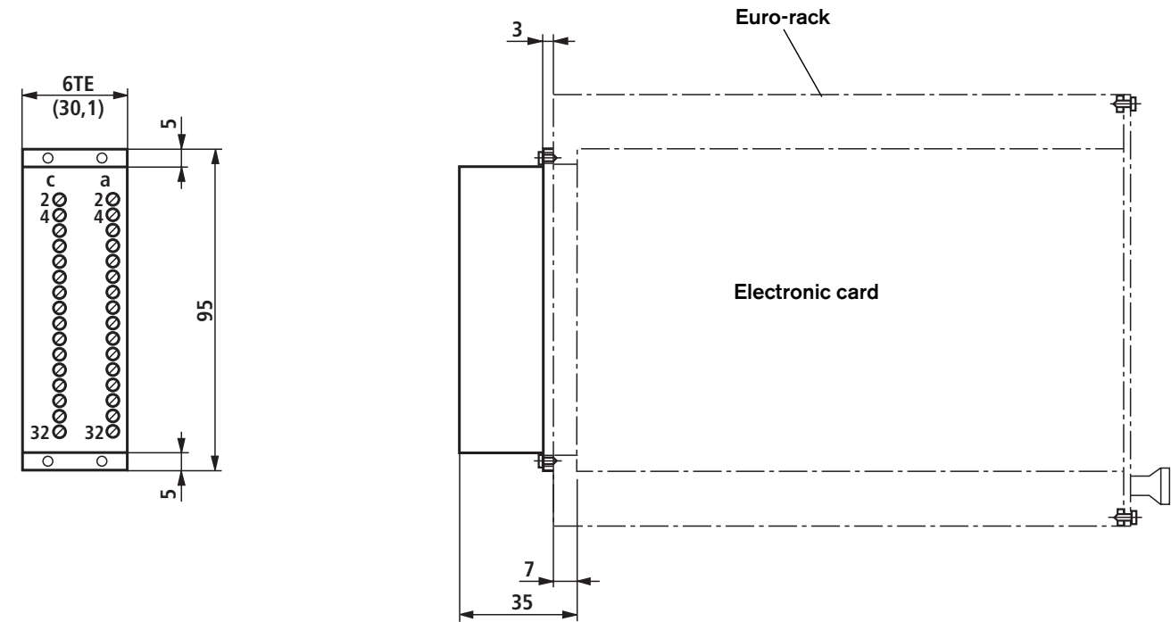
Adapter, 32-pin, form D
