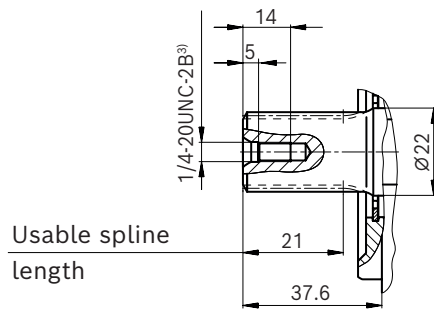
Connection table A10VZG
