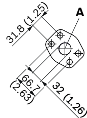
Detail W
