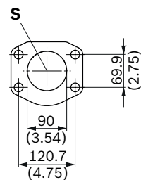
Detail W
