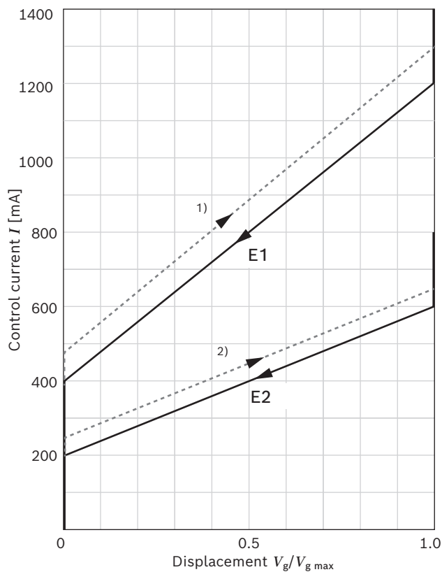
▼ Characteristic curve E1/E2
