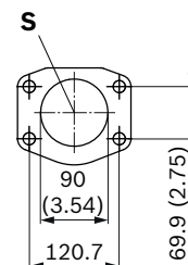
Detail W
