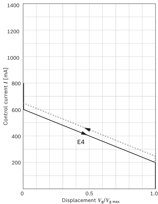
▼ Characteristic curve E4
