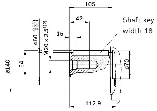
B4 – Ø60 A 18x11x100
